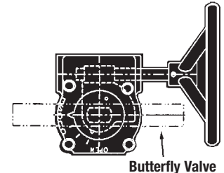
Gear Operator
